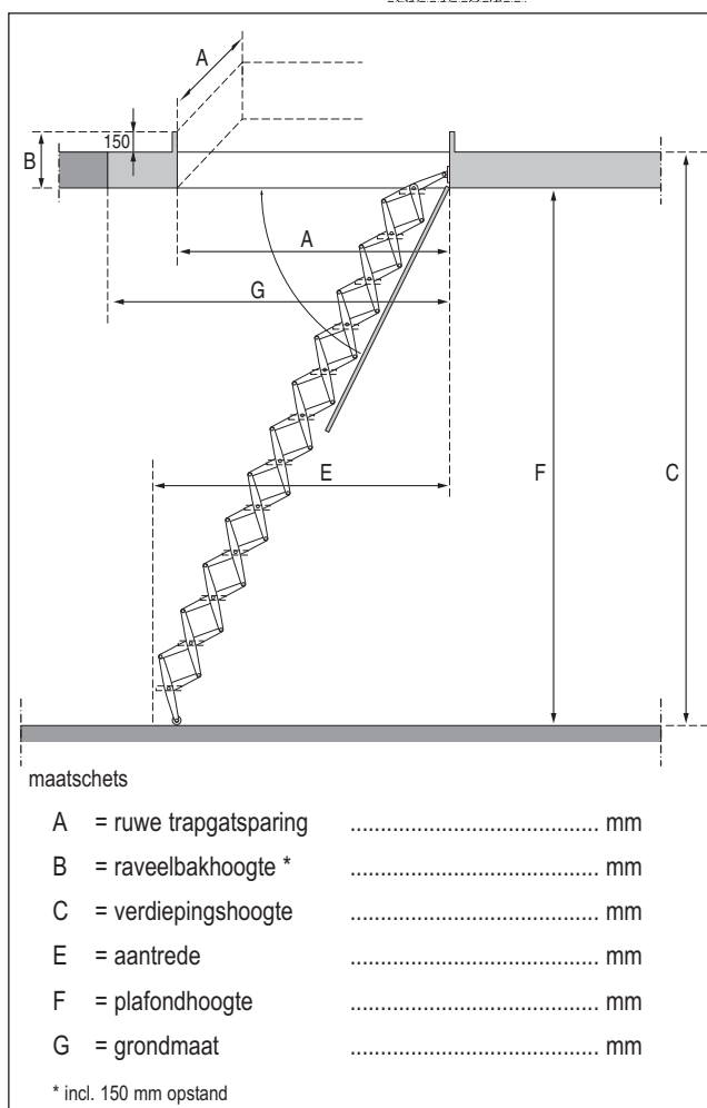
type 2470 geopend
